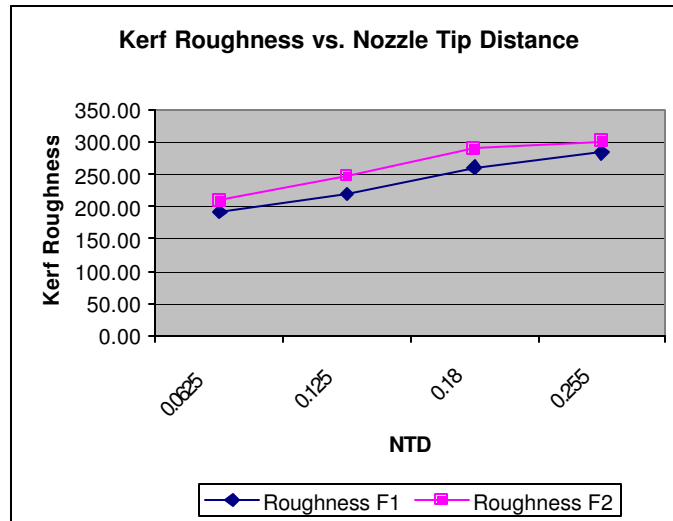
Figure 7. Kerf Roughness vs. NTD
