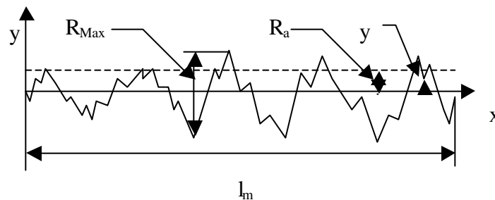
Figure 4. Kerf Roughness Measurement.
